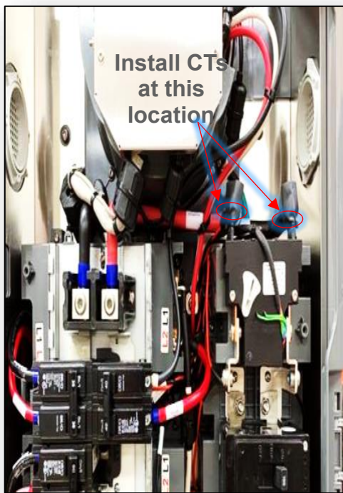
Figure 3: PCS CT placement location inside Enpower
